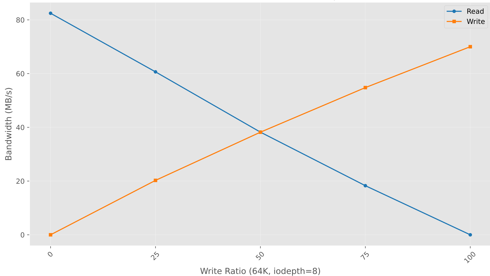
Bandwidth vs Write Ratio (64K, iodepth=8)
